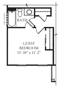
Partial First Floor plan at Opt. Guest Bedroom - Federal
