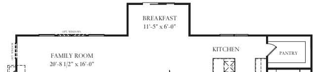
Partial First Floor at Opt. 6' Breakfast Extension
