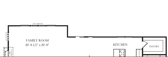
Partial First Floor at Opt. 4' Family Room Extension
