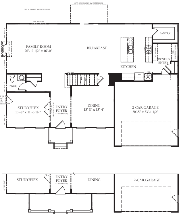
Partial First Floor at Opt. 3/4 Porch - Federal
