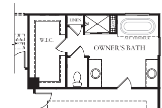
Partial Second Floor Plan w/ Opt. 5-piece Owner's Bath
