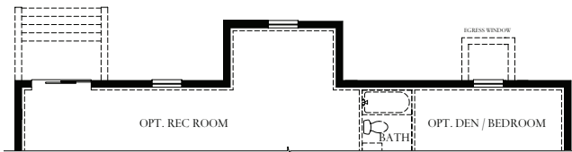
Partial Lower Level at Opt. 6' Breakfast Extension
