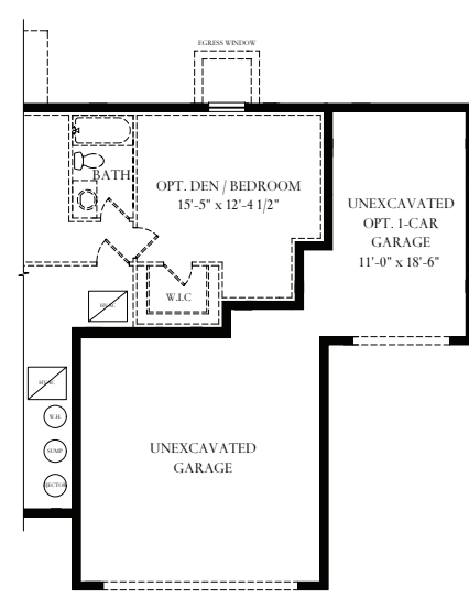
Partial Lower Level at Opt. 1-Car Garage w/ 2-car Front Load Garage
